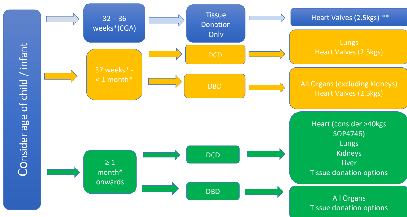
Figure 1: Screening Flowchart
